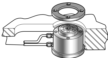
"Floating" Cylinder
